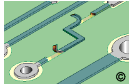
Evaluate the damage and measure the conductor width
