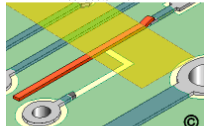
Remove the damage, place the new Track and solder one end.
