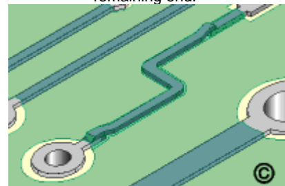
Bond in place and overcoat with epoxy.
